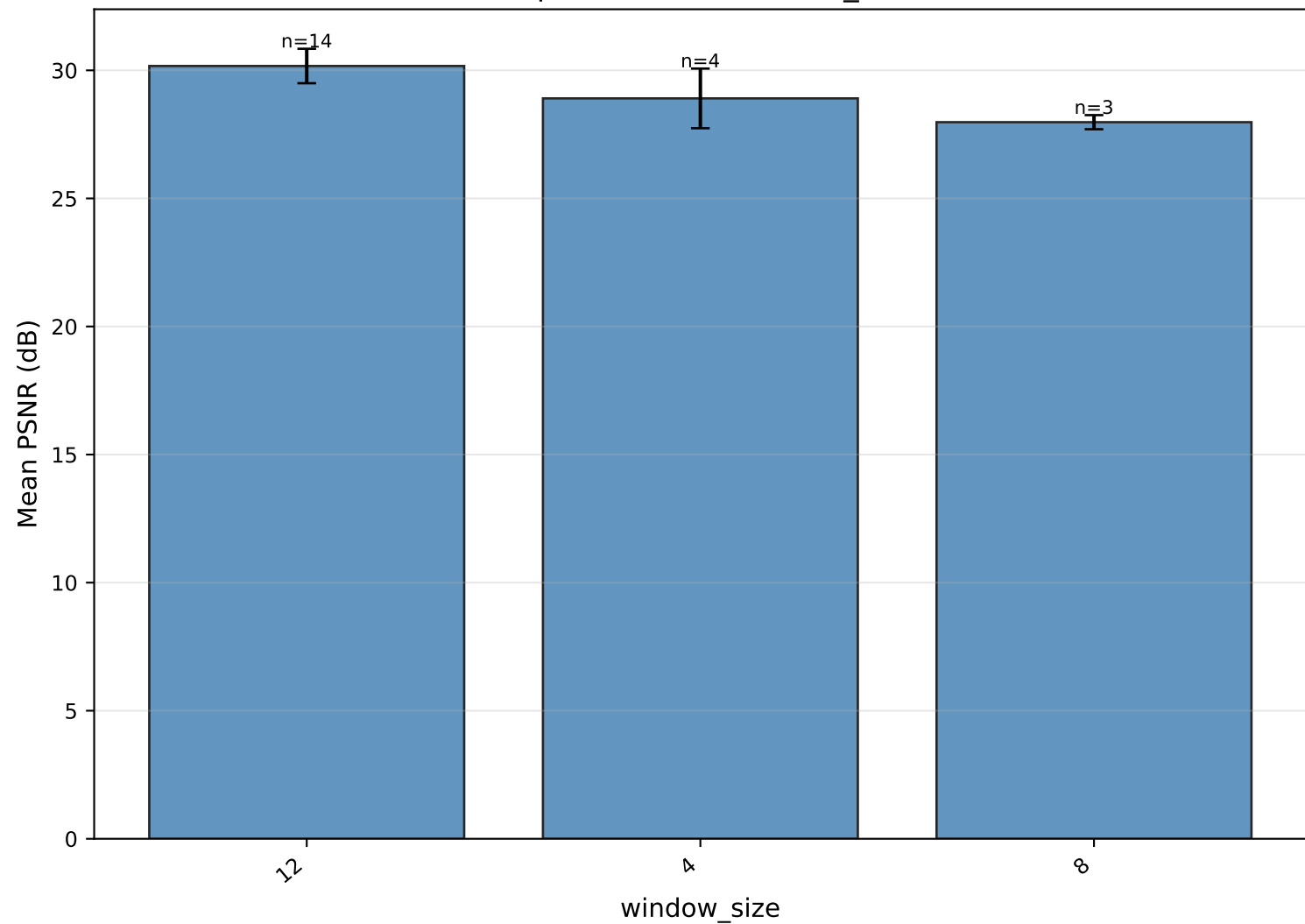
Mean PSNR per value of window_size — ELAN
